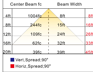
200W/90D
