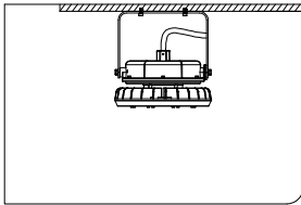
Ceiling Bracket Mounting
