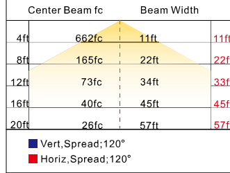
200W/120D
